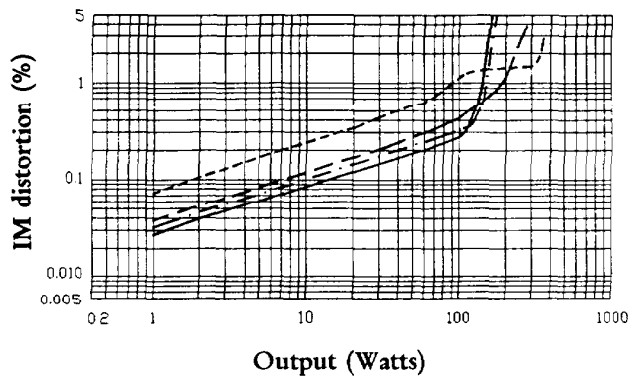
INTERMODULATION DISTORTION vs. OUTPUT
