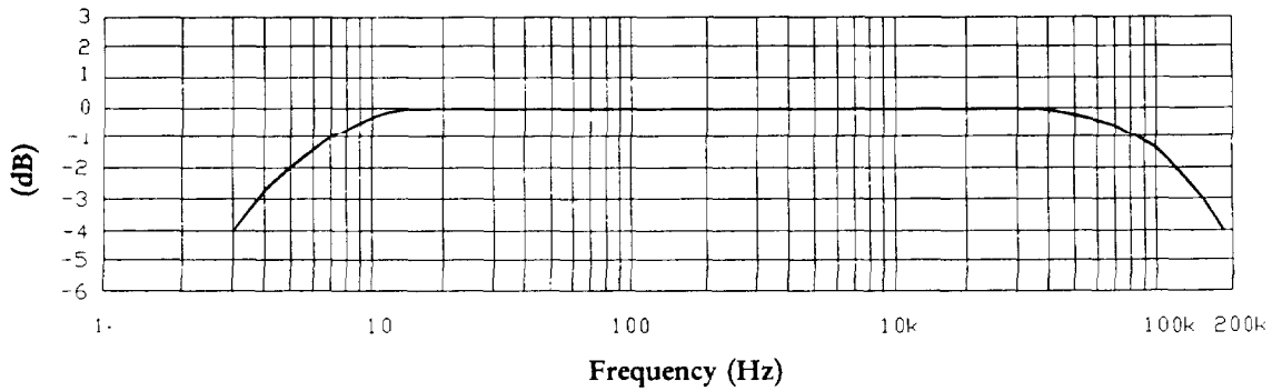
FREQUENCY RESPONSE
